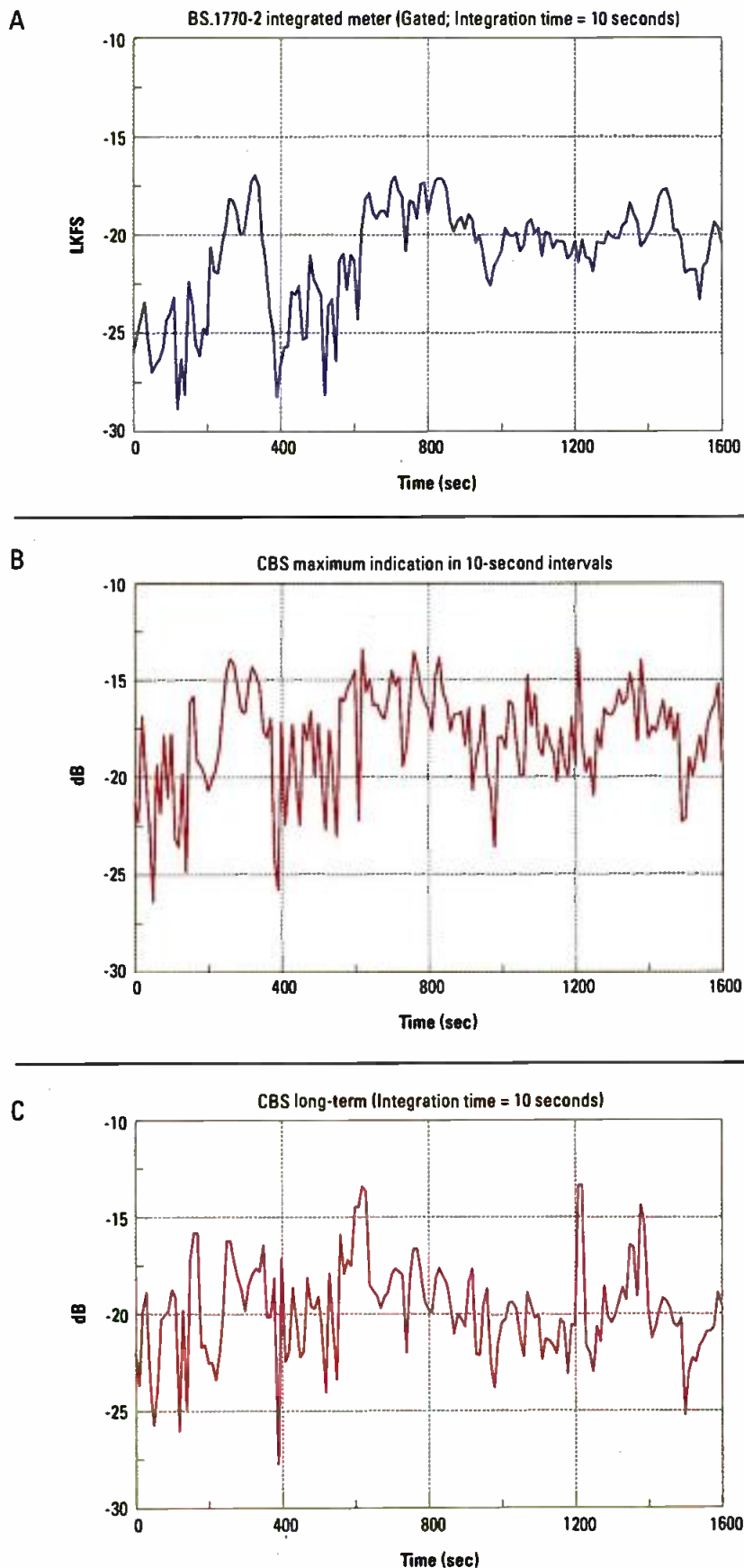
Figure 1: This shows unprocessed input and the peak output of the BS.1770 and CBS Loudness Meters in each 10-second interval as a function of time.
