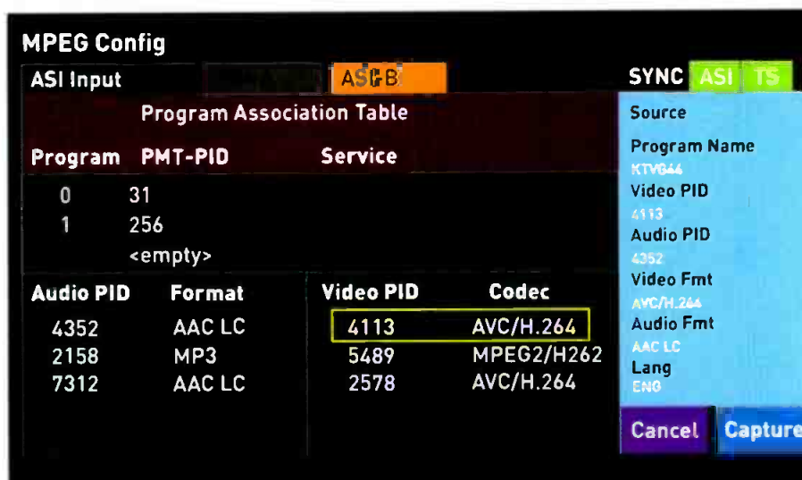
Figure 1. Multiplatform operations often use lower-cost monitoring systems to check for faults at key points in the transmission path. One such point is analysis of MPEG errors — including missing stream PIDs — capable of preventing user devices from properly decoding content.
